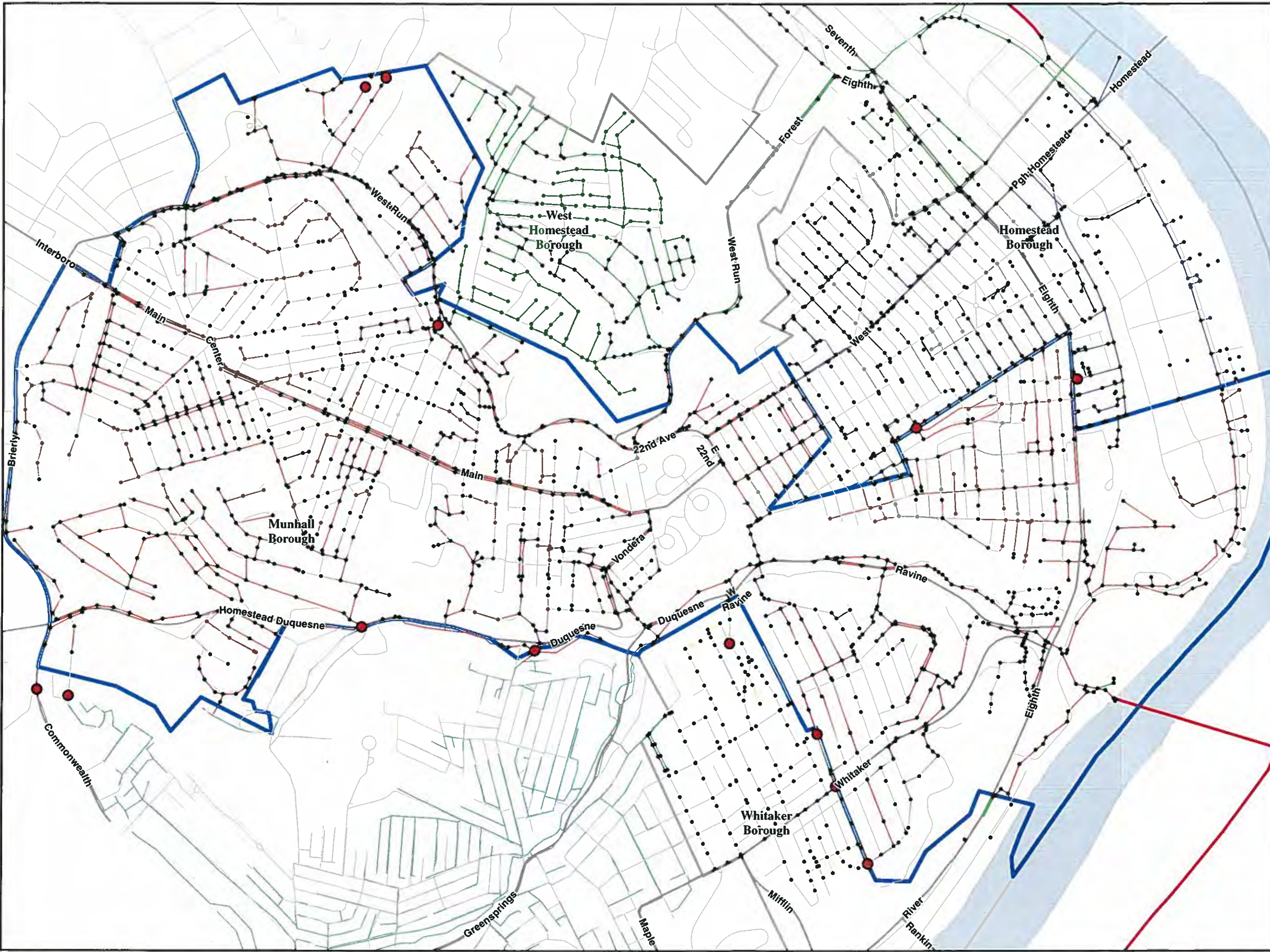
Figure 3: Munhall Sanitary Sewer Municipal Authority Service Area
