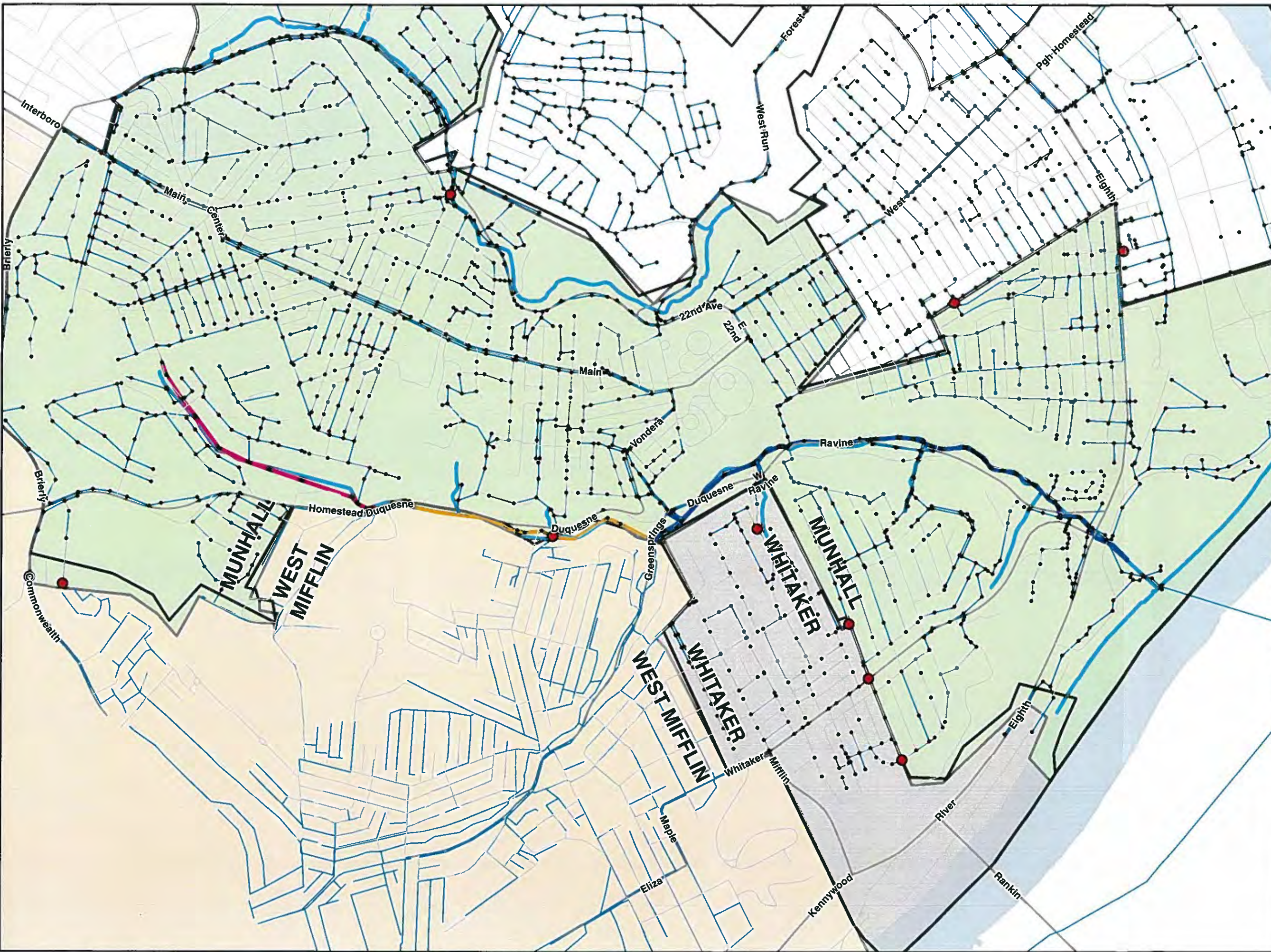
Figure 6: Homestead Run Interceptor
