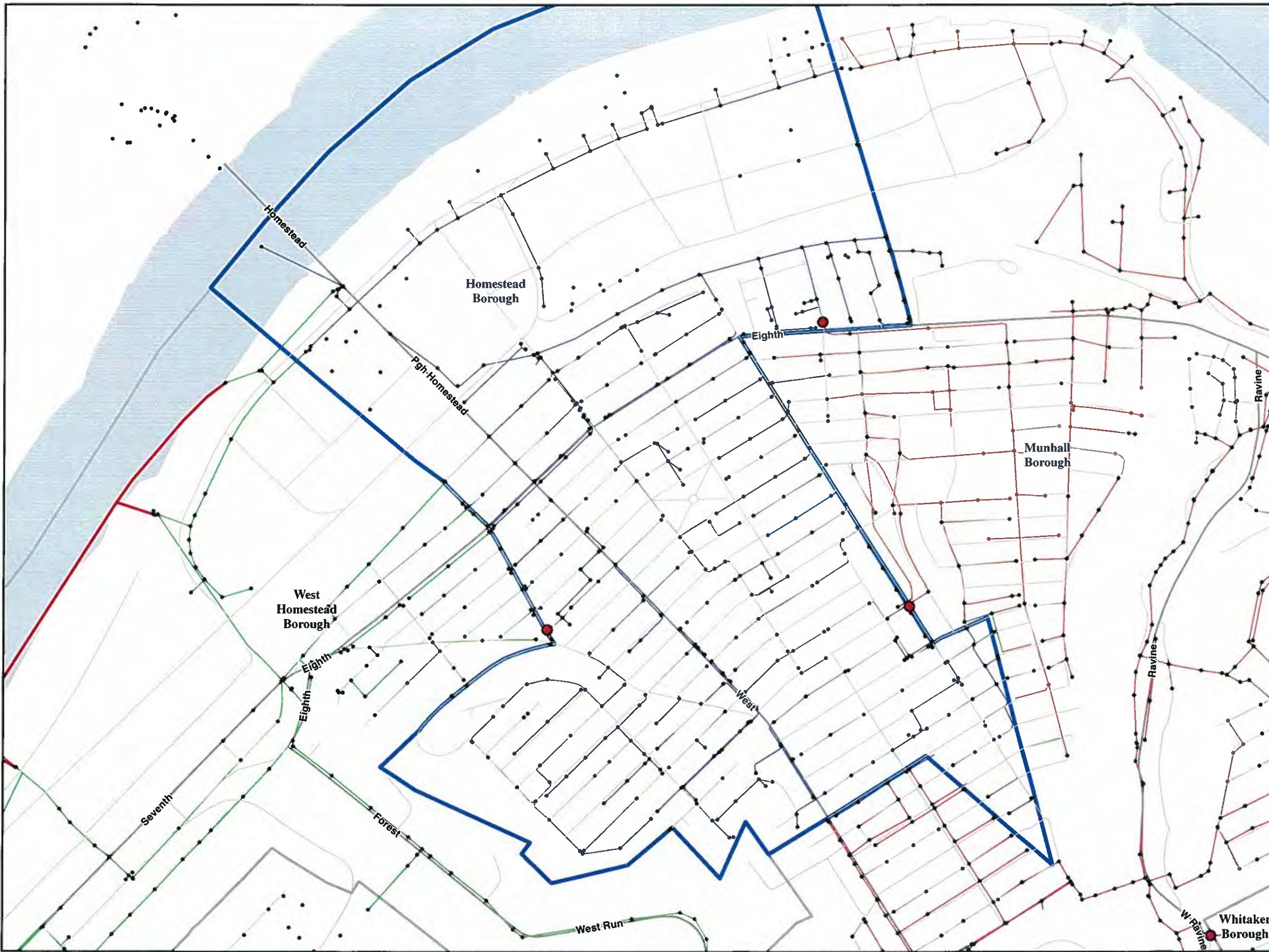
Figure 2: Homestead Borough Service Area
